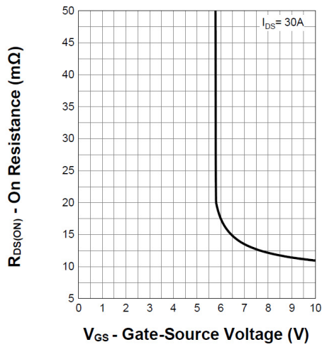
Fig 7. Transfer Characteristics
