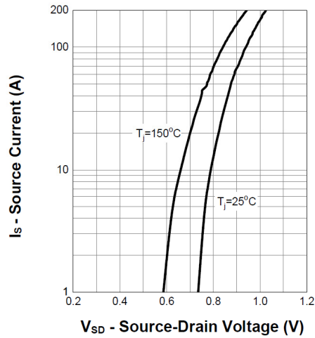
Fig 10. Diode Forward Current
