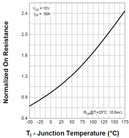
Fig 9. Normalized On Resistance
