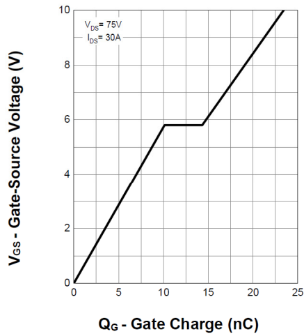
Fig 12. Gate Charge
