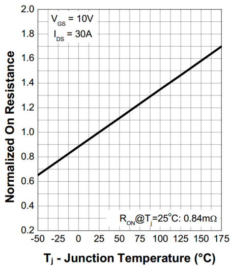
9. Normalized On Resistance
