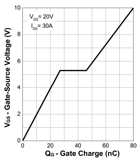
12. Gate Charge
