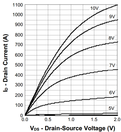
5. Output Characteristics
