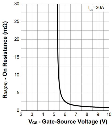
7. Transfer Characteristics
