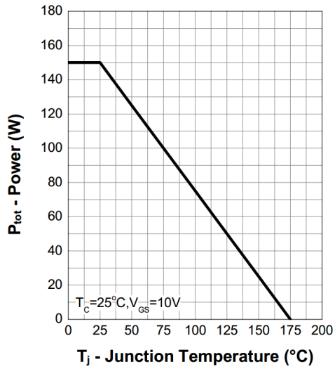
1. Power Capability
