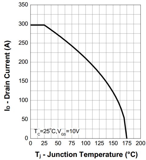
2. Current Capability
